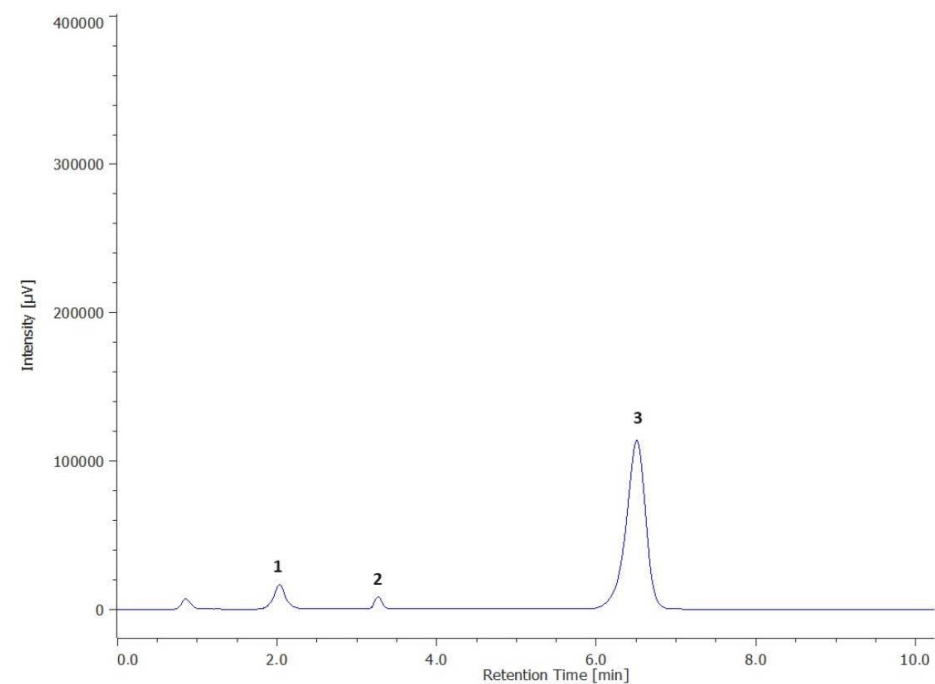
Figure 1. Chromatogram of vitamin E quantification. (1— \alpha -tocopherol; 2— \beta -tocopherol; 3—tocol-internal standard).
