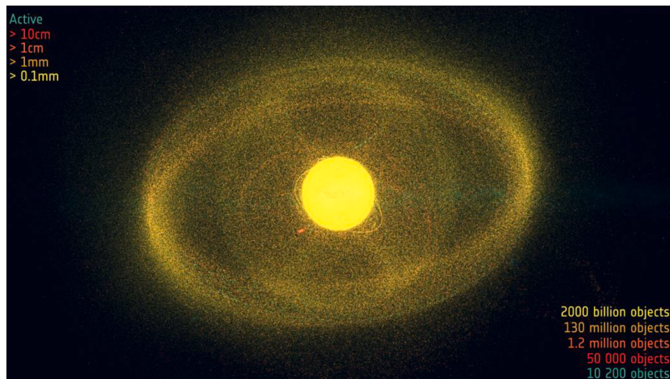
Fig. 1. Overview of space debris distribution around the Earth (Source: [11]).
