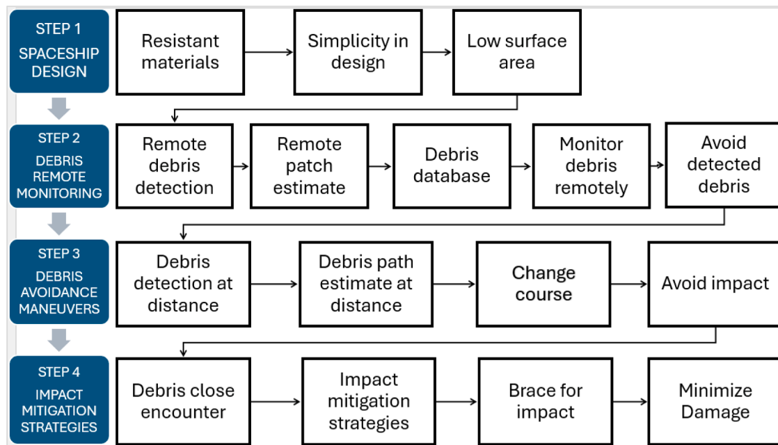
Fig. 2. Proposed strategy for minimising space debris risks (Source: Authors).
