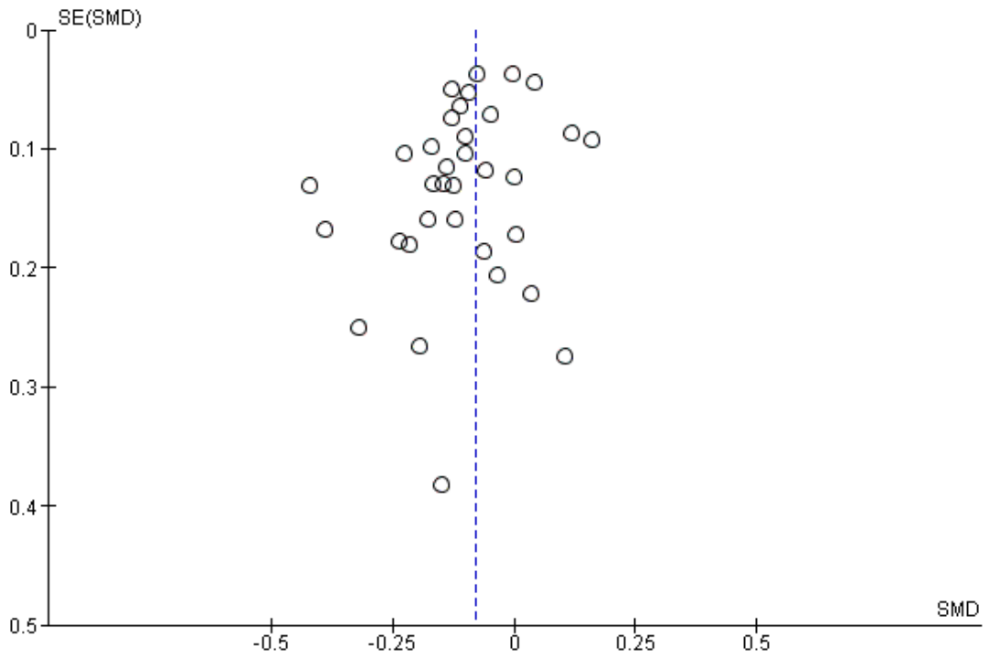
Figure 6. Funnel plot of comparison: I Social norms (SN) vs control, outcome: I.6 Quantity of drinking: 4+ months.
